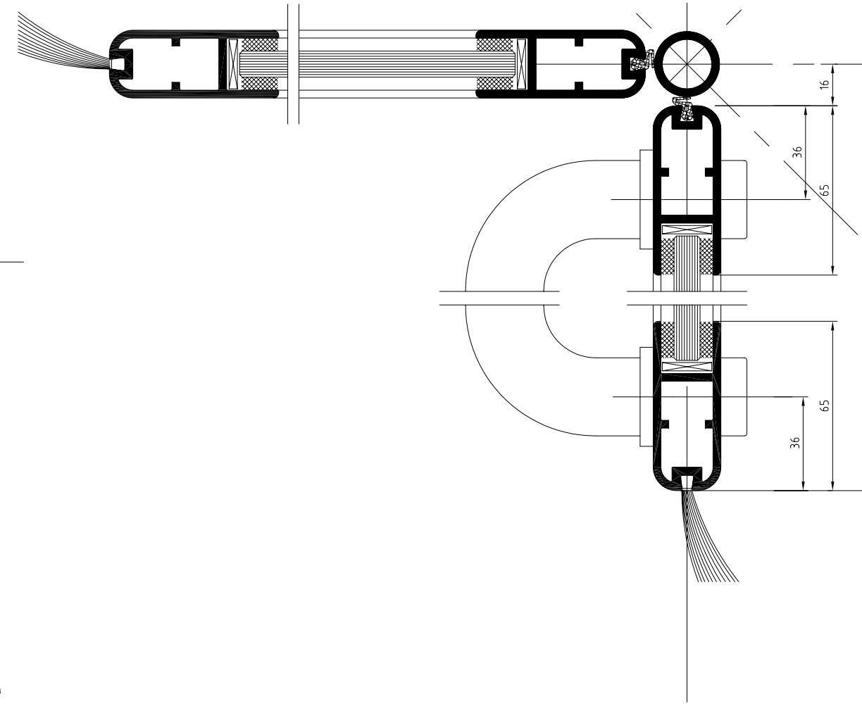
DETAIL E
